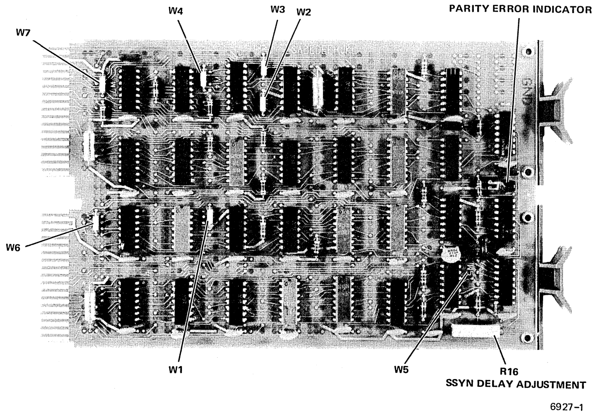
Figure 5-14 M7259 Parity Control Module
