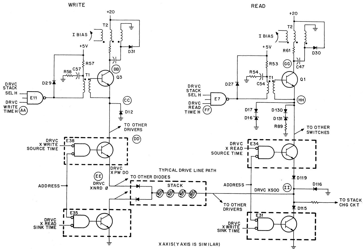
Figure 5-8 Typical Read/Write Drive Circuit
