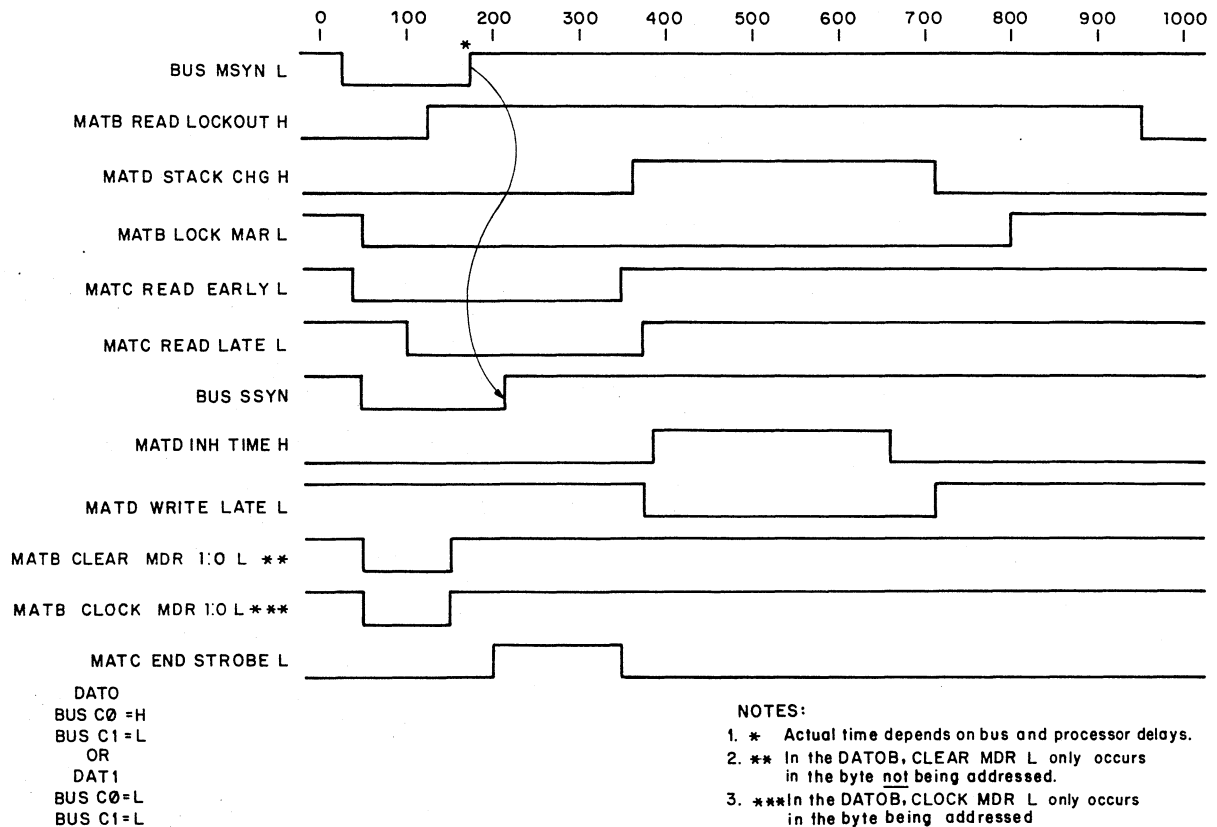
Figure 2-7 DATO, DATOB Mode Timing Diagram
