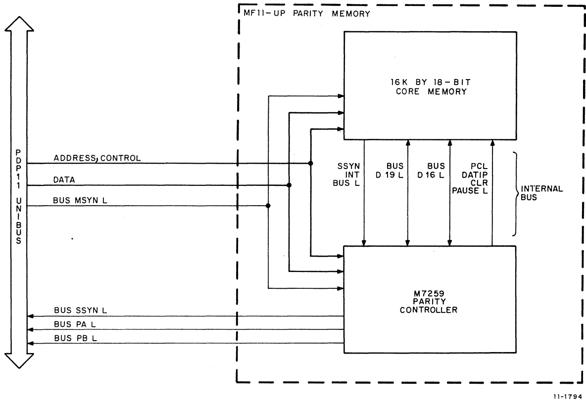
Figure 4-2 Parity Controller Block Diagram
