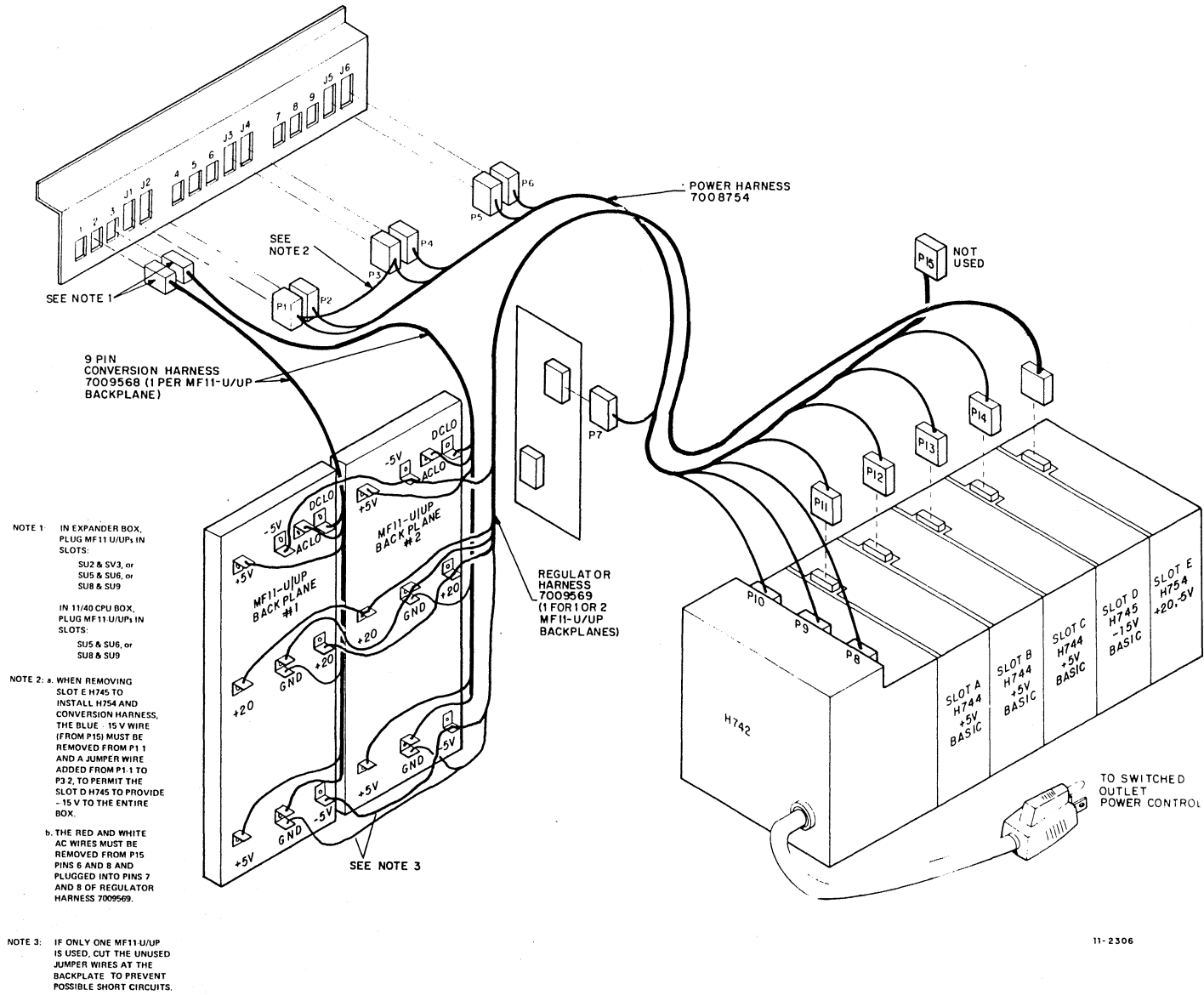
Figure S-2 Early MF11-U Power Distribution System
