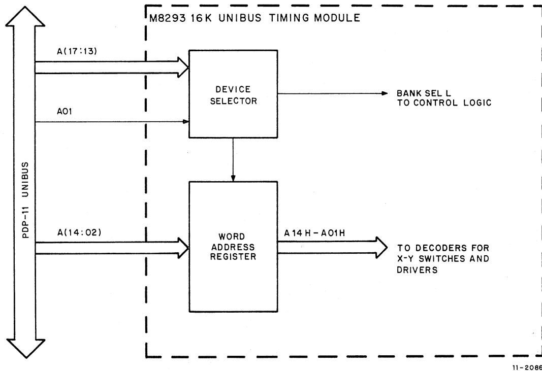
Figure 2-10 Device and Word Address Selection Logic Block Diagram
