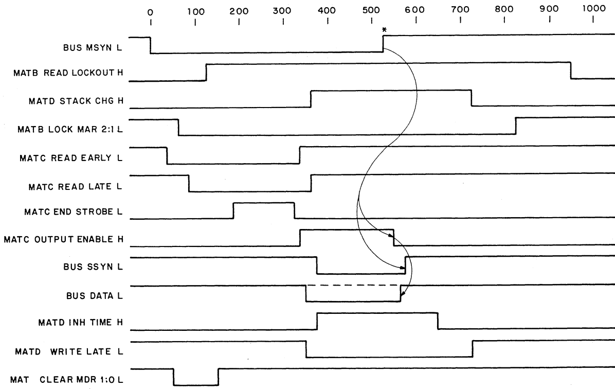
Figure 2-5 DATI Mode Timing Diagram
